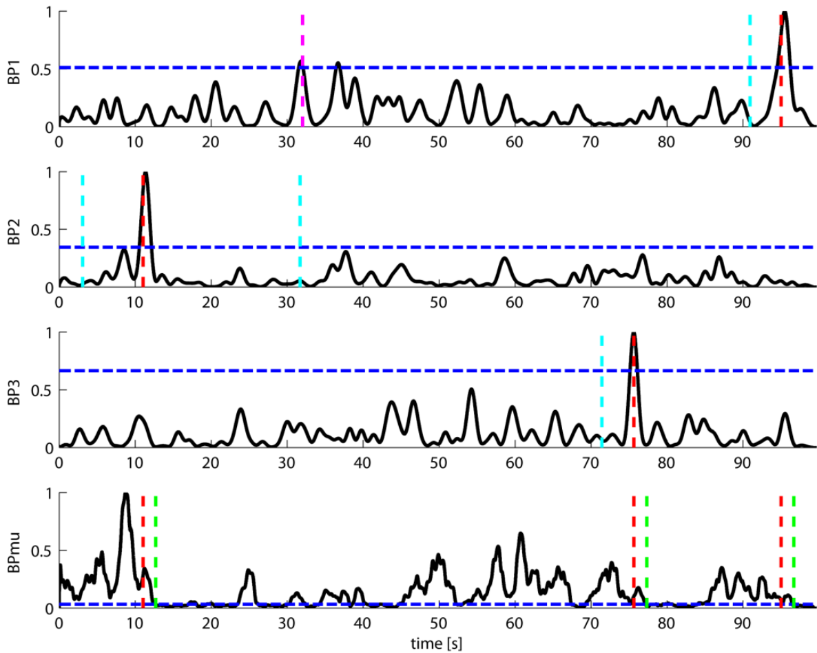
Figure 7.8 - Normalized band-powers FBP_1 , FBP_2 , FBP_3 and FBP_{\mu} from top to the bottom. Three successful trials (TP), one per each LED, and one false activation of SSVEP-BCI ( FP_{ssvep} ) for subject S5, during the representative 100 seconds interval are presented. Subplot arrangement and color codes for turquoise, red, blue, and green are the same as in Figure 7.7. Pink vertical dashed line marks one incorrect SSVEP detection when subject reached and focused on the second object ( LED_2 ) but the detection falsely occurred in FBP_1 (threshold TH_1 was exceeded by FBP_1 for DT_s ). Taken from [124].
